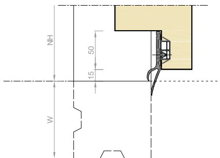
DETAIL 4: +°C
