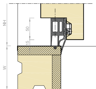
DETAIL 4: -°C
